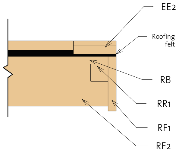
3) Roof Reinforcement
