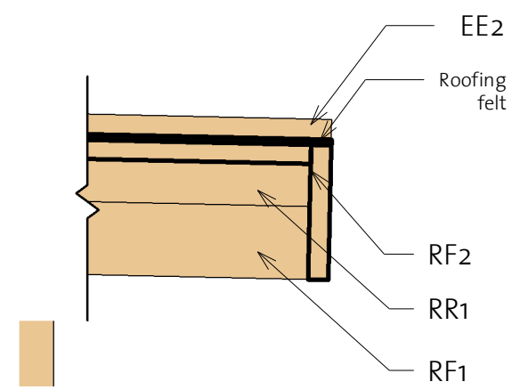
3) Roof Reinforcement
